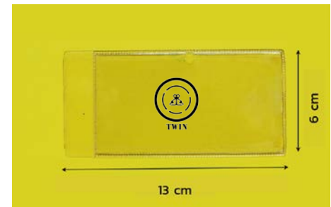
NOREN TAG T009 :6 x 13 cm thickness 0.25 mm Plastic case
